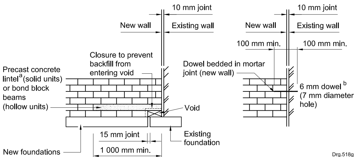
a) Foundation detail
