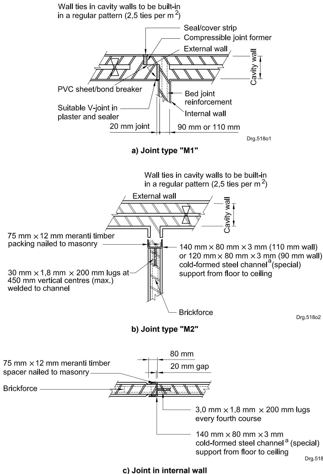
Figure A.6 — Full movement joint details for buildings with external cavity walls
