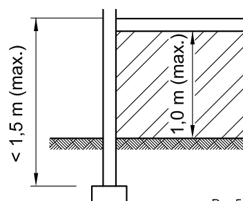
c) Maximum heights of fill and foundation wall
