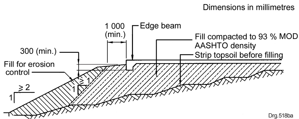
a) Slab-on-the-ground foundation founded on engineered fill
