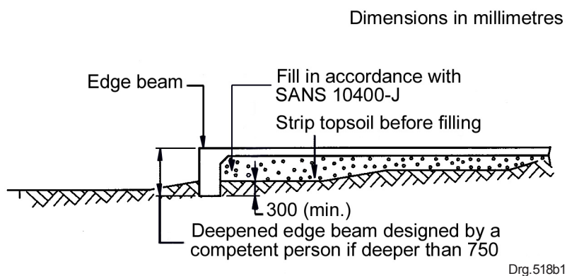
a) Fill under slab-on-the-ground foundation
