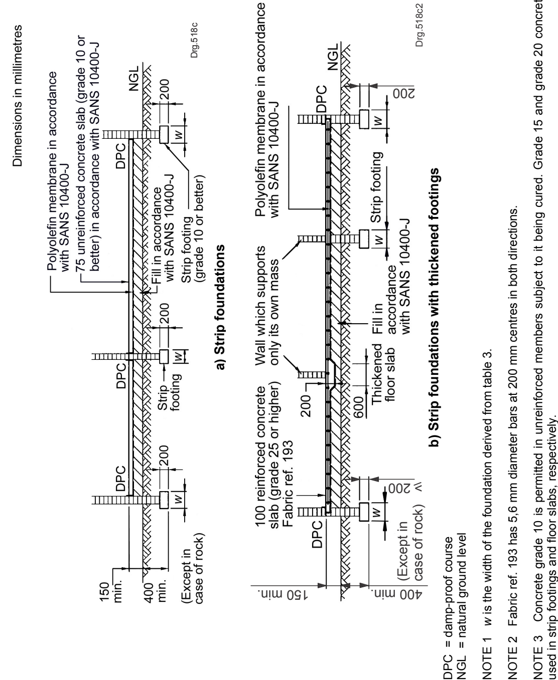
Figure 5 — Strip footing details (class C, H, R and S sites)
