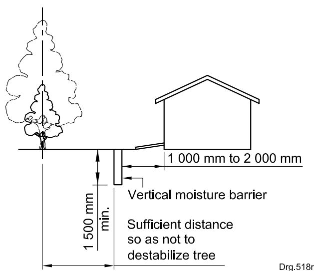
Figure D.1 — Vertical moisture barrier
