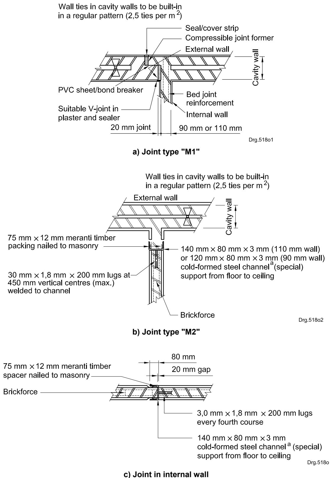
Figure A.6 — Full movement joint details for buildings with external cavity walls
