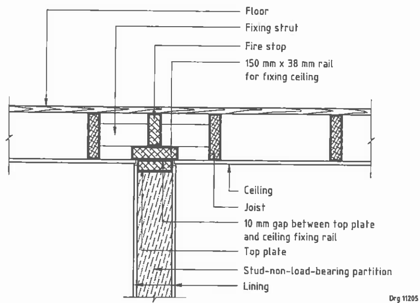
Figure 29 — Attachment of non-load-bearing wall to first floor framing
