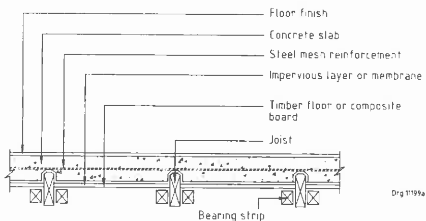
Figure 16 — Bathroom floor construction for tile covering
