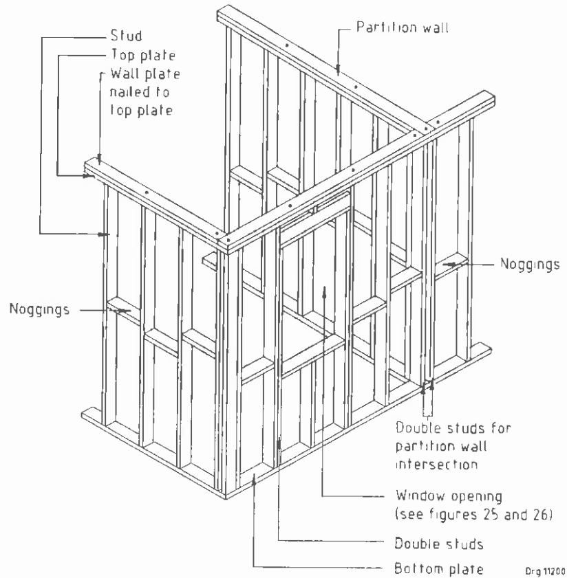
Figure 18 — Platform construction
