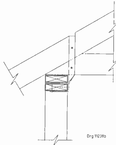
b) Strap to top plate — Truss not directly over stud
