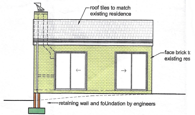
1:100 south east elevation
