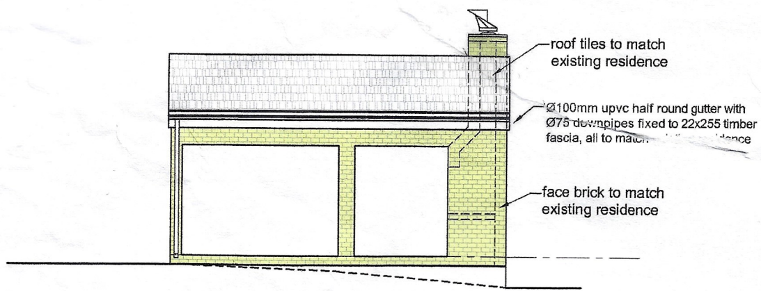
1:100 north west elevation
