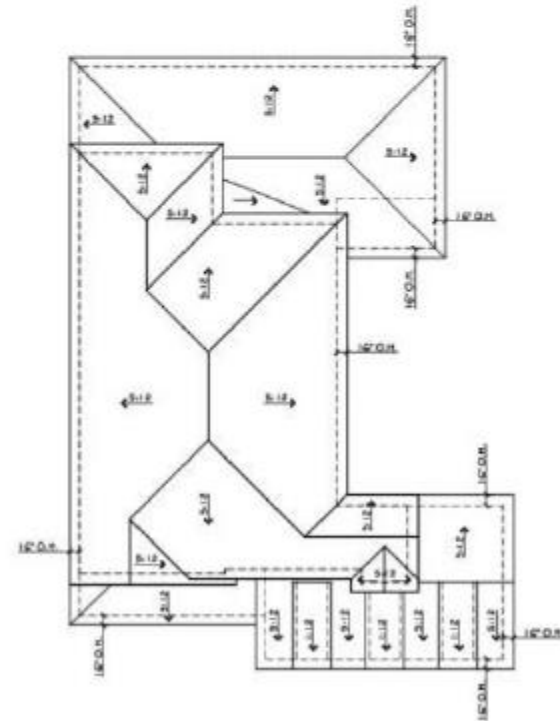
ROOF PLAN
