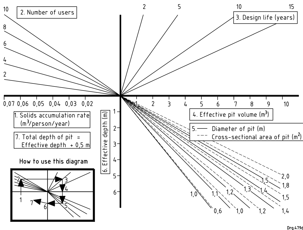
Figure B.2 — Nomogram for determining the required pit depth
