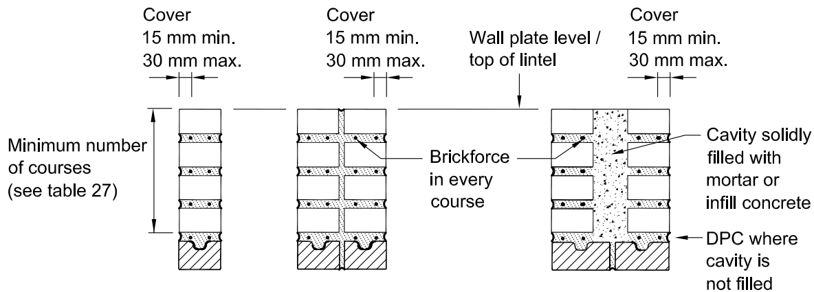
a) Section through lintels
