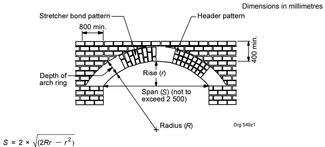
Figure 33 — Masonry arches
