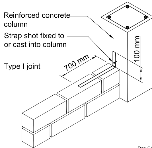
a) Isometric view of fixing to column (type I joint)
