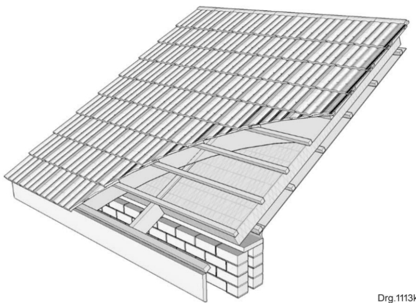
Figure F.5 — Tiled roof with reflective foil insulation installed over rafters with 38 mm airgap (brandering) and rigid bulk insulation fixed to underside of the rafters
