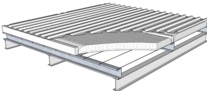
Figure F.3 — Bulk insulation installed over purlin with continuous solid spacer
