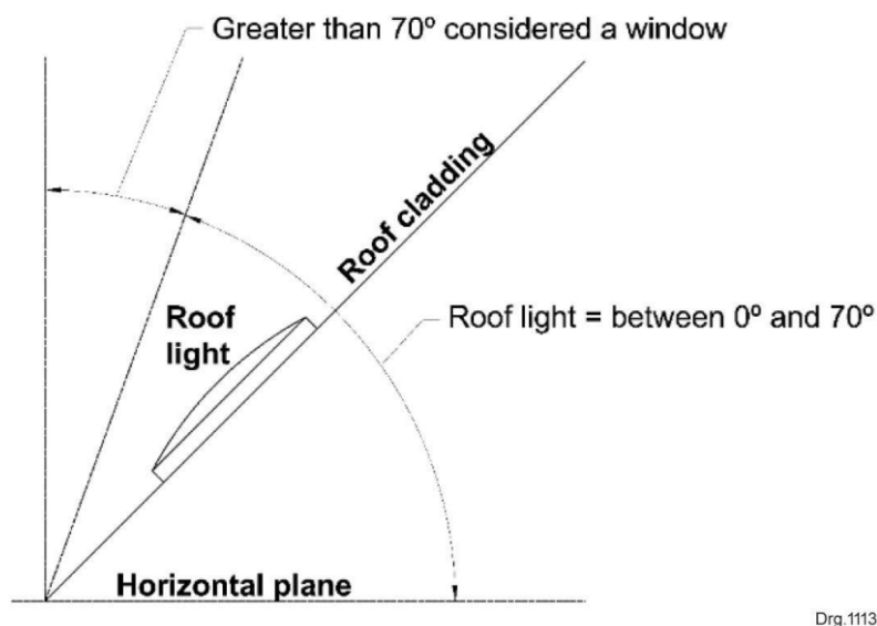
Figure 6 — Defining a roof light
