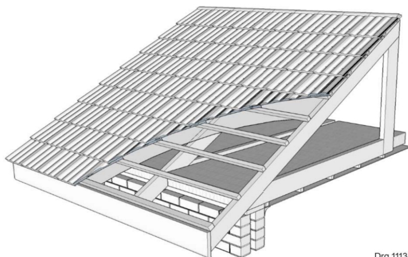
Figure F.4 — Tiled roof with reflective foil insulation installed over rafters with 38 mm airgap (brandering) and rigid bulk insulation installed on top of ceiling
