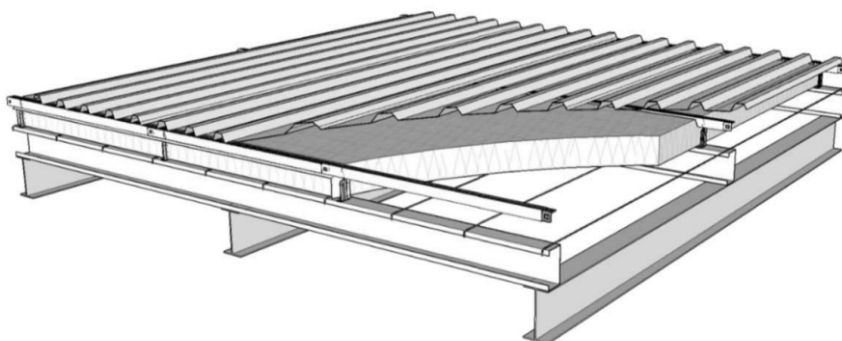
Figure F.2 — Bulk Insulation installed over purlin with mechanical spacer
