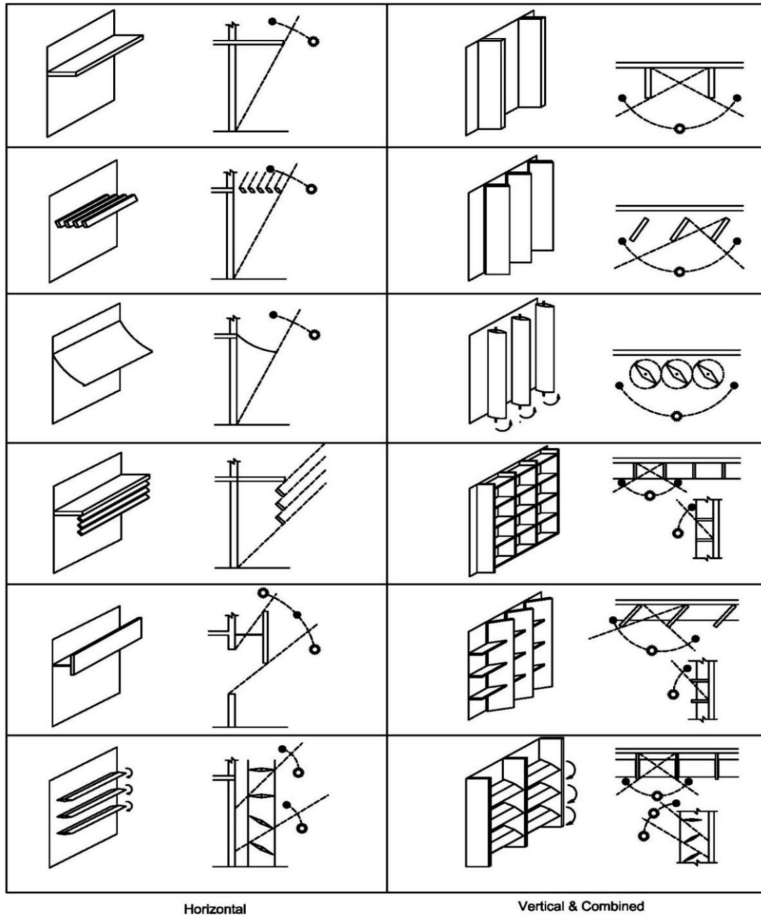
Figure D.1 — Shading devices
