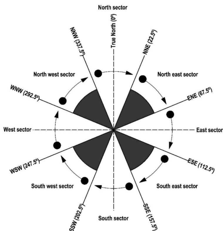
Figure 2 — Orientation sectors
