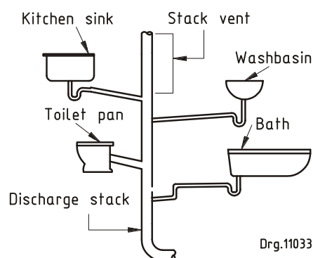
Figure 6 — Single-stack system
