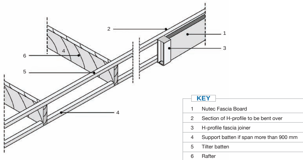
Fig 2 : Additional Support Required For Nutec Fascia Boards Where Distance Between Rafters Exceeds 900 mm
