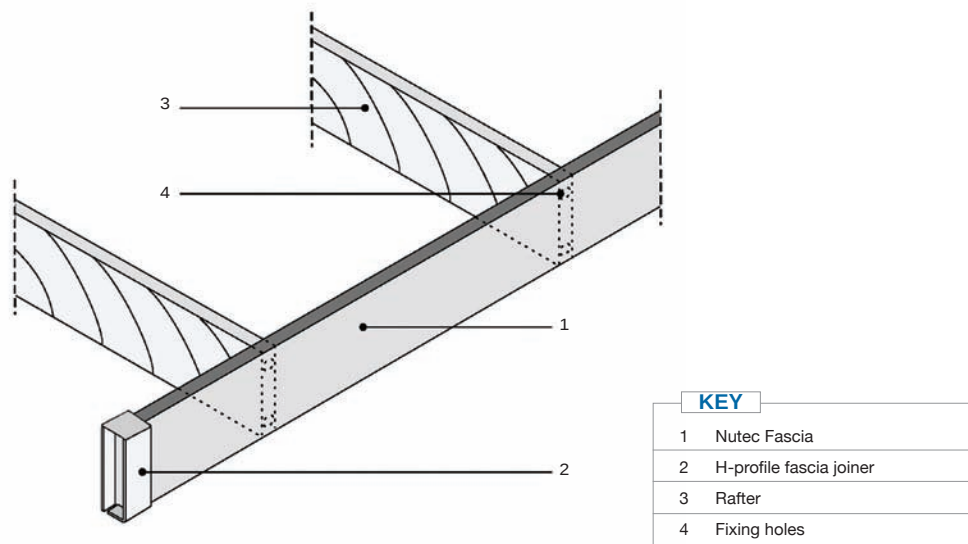
Fig 1 : Normal Fixing without additional support structure
