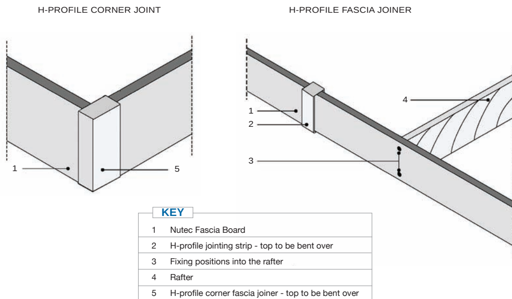
Fig 3 : Joint Detail Using H-Profile Fascia Joiners
