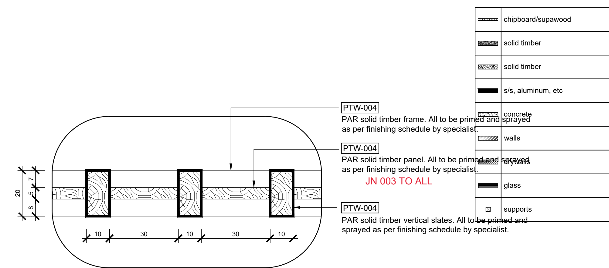
detail 1 scale 1 : 1
