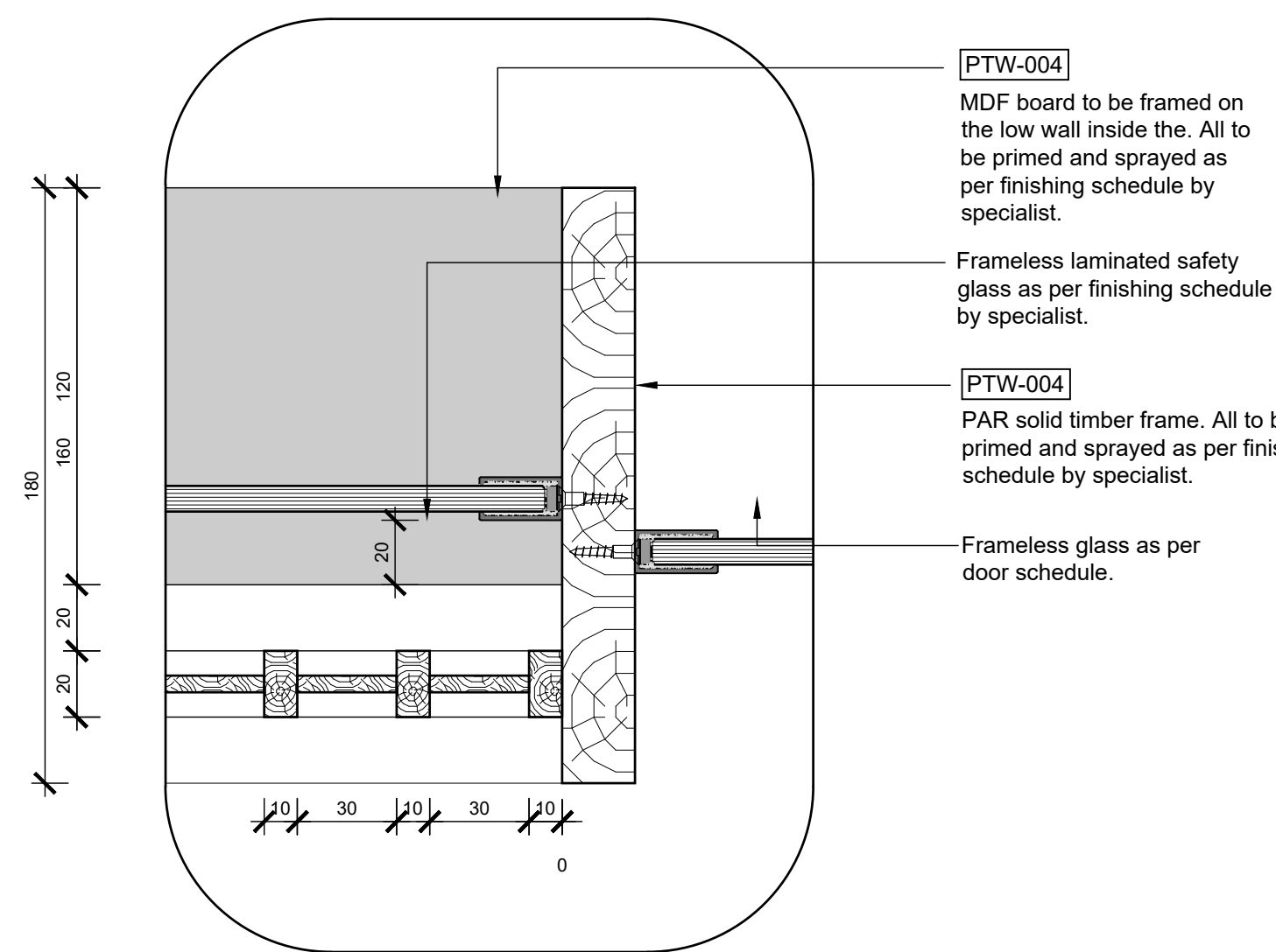
detail 3 scale 1 : 2
