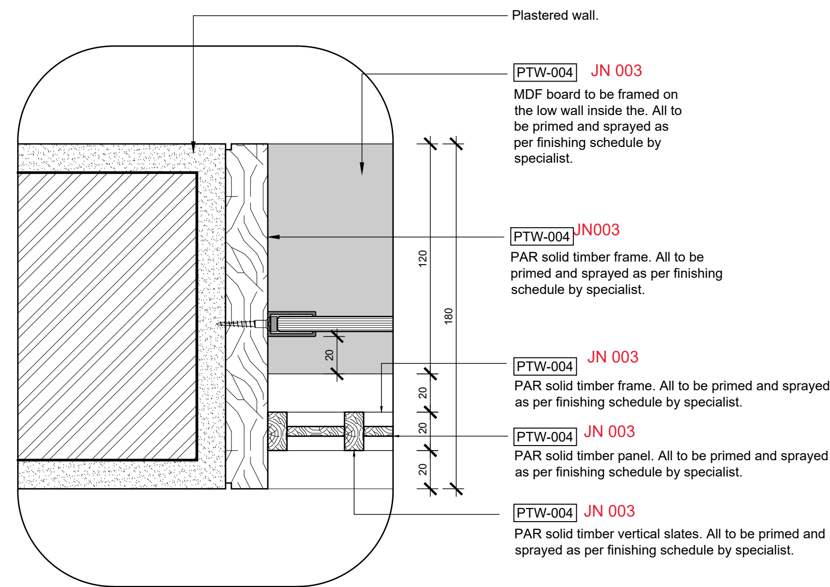
detail 2 scale 1 : 2
