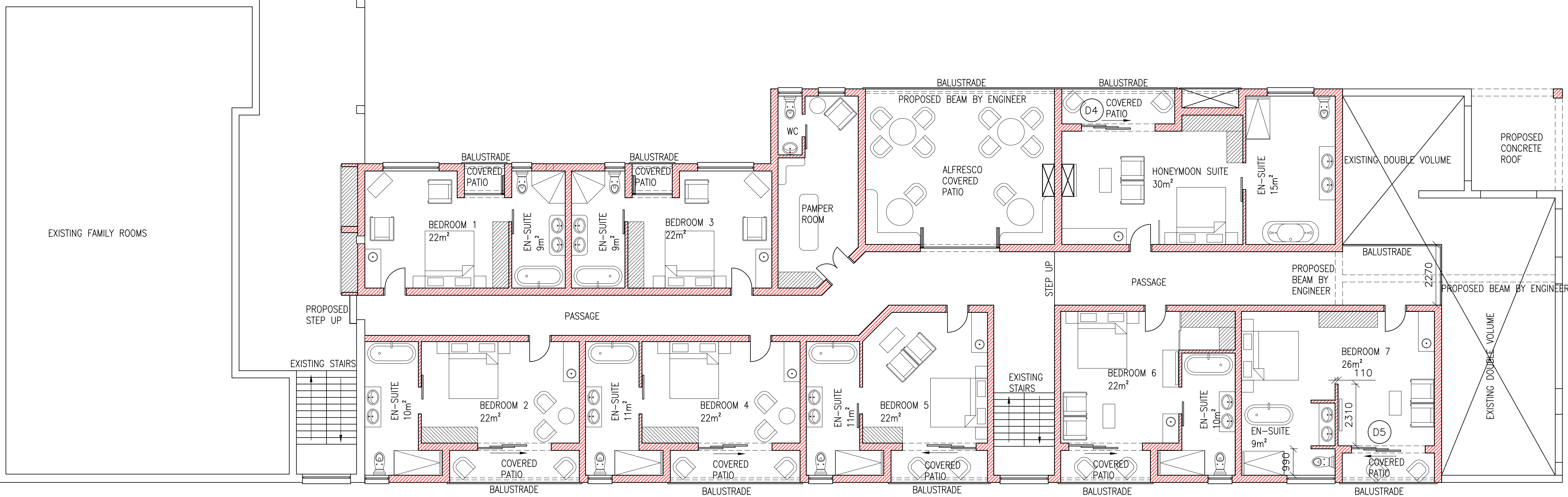
FIRST STOREY PLAN SCALE 1:100
