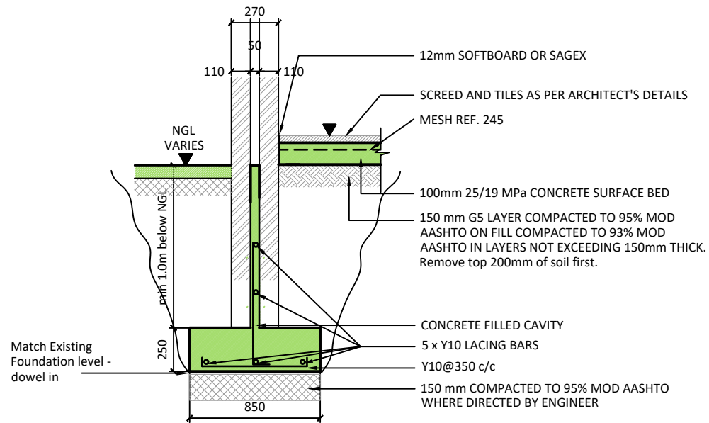
TYPICAL FOUNDATION (270 WALLS)
