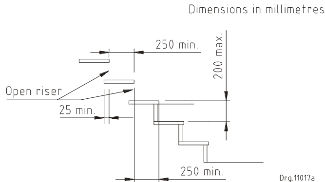
Figure 2 — Dimensions of treads and risers on a stairway
