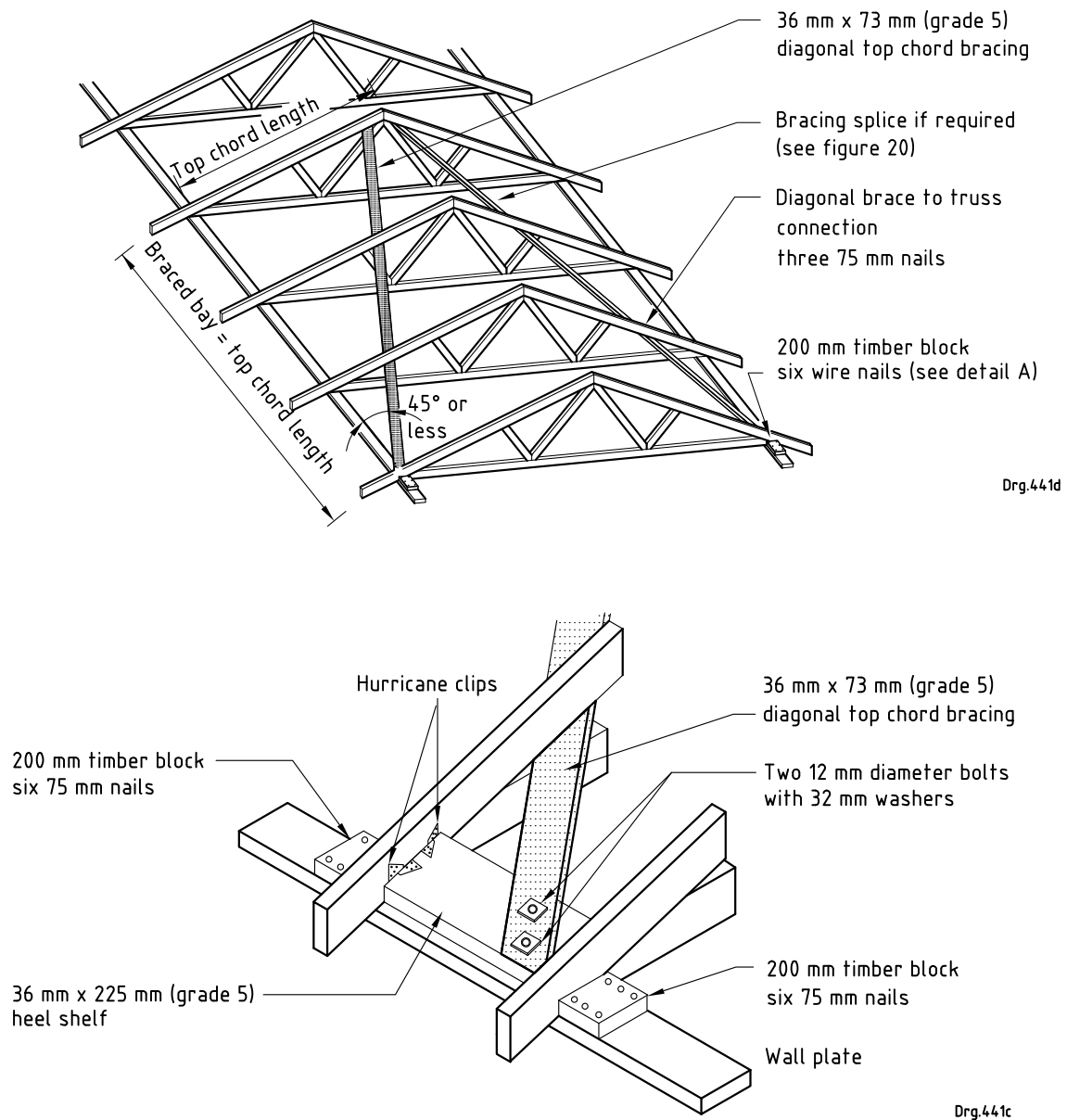
Detail A
