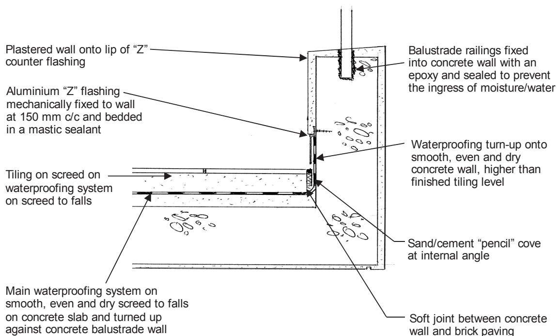
Figure A.3 — Waterproofing turn-up detail at concrete balustrade wall on balcony or against concrete wall
