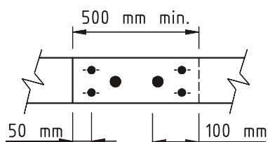
a) Splice detail
