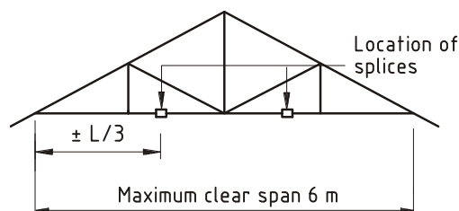
b) Double-pitched four-bay Howe truss
