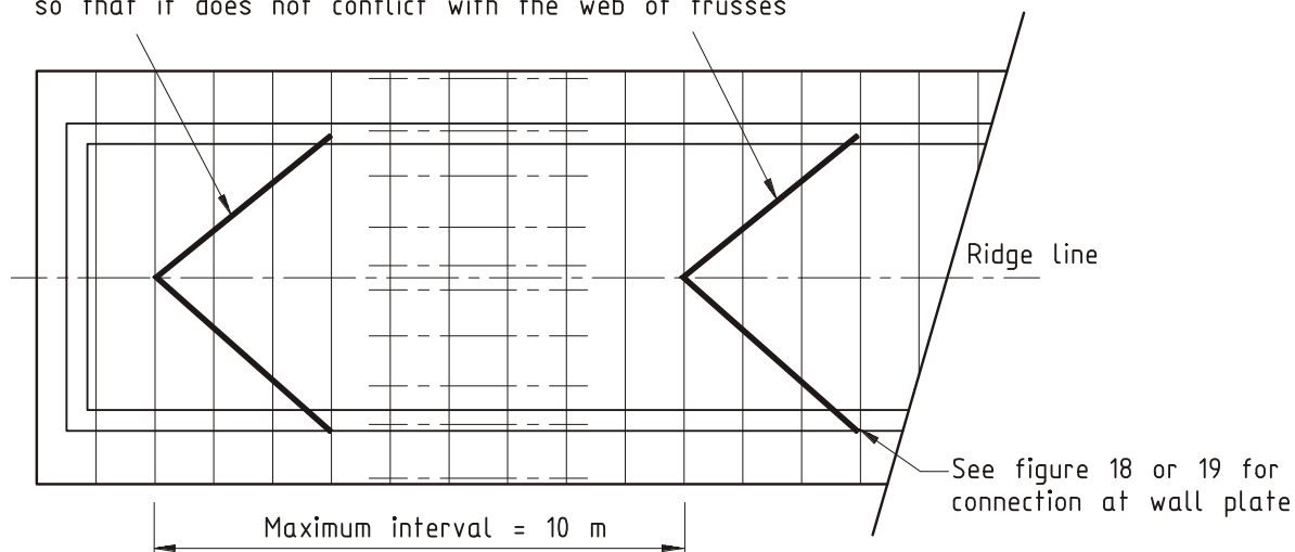
Plan on top chords
