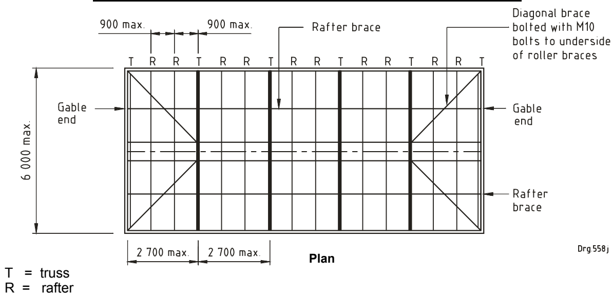
Figure 29 — Truss for thatch roofing in gable-to-gable rectangular buildings that have a clear span that does not exceed 6,0 m
