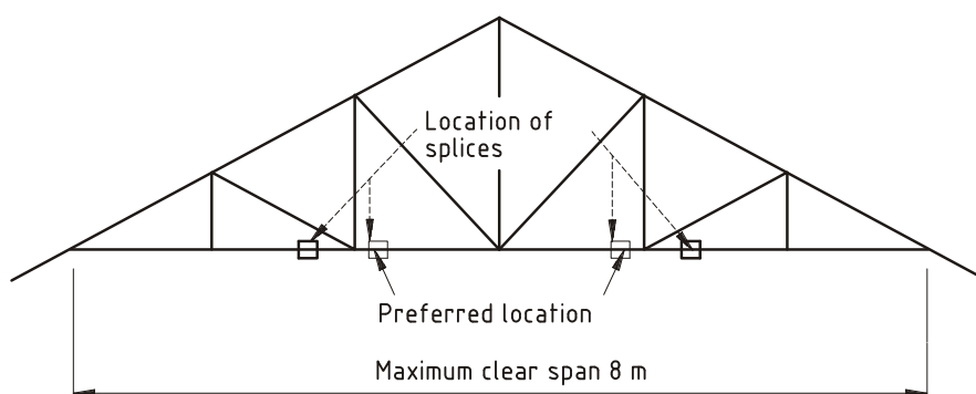
c) Double-pitched six-bay Howe truss
