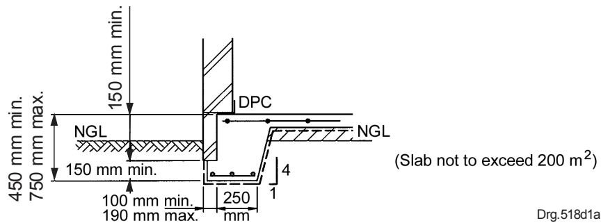
b) Deepened edge rebate detail
