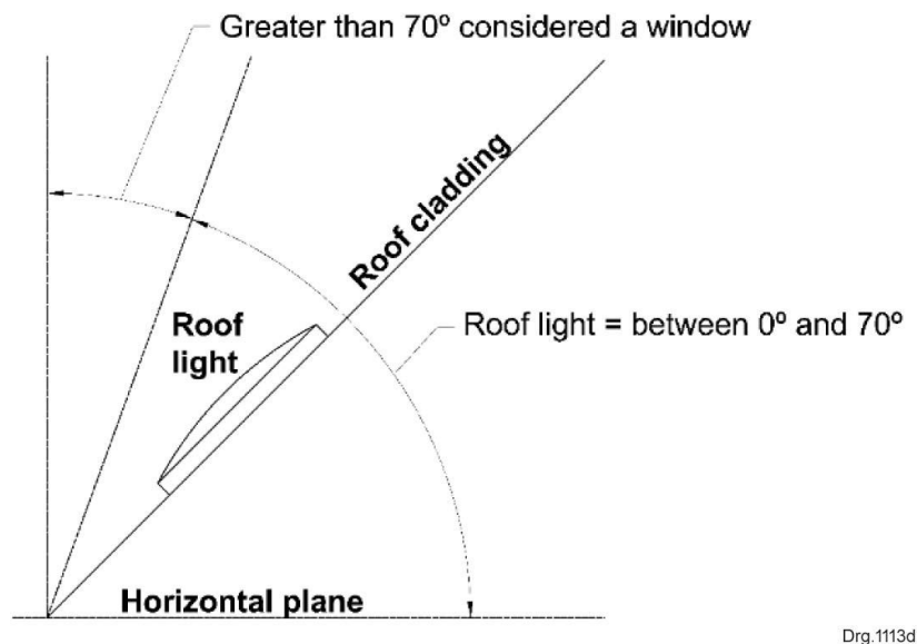
Figure 6 — Defining a roof light
