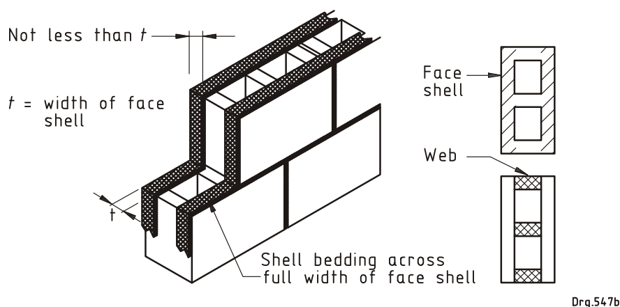
Figure 3 — Shell bedding
