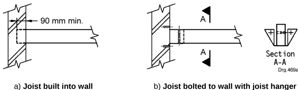
Figure 1 — Bearing details for suspended timber ground floors
