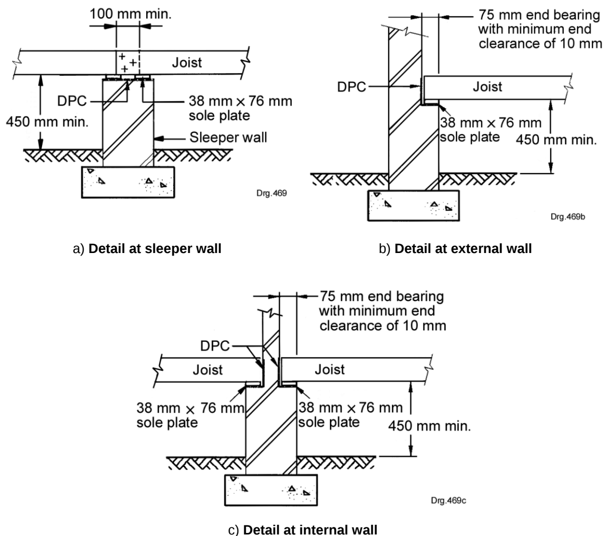
Figure 1 — Bearing details for suspended timber ground floors
