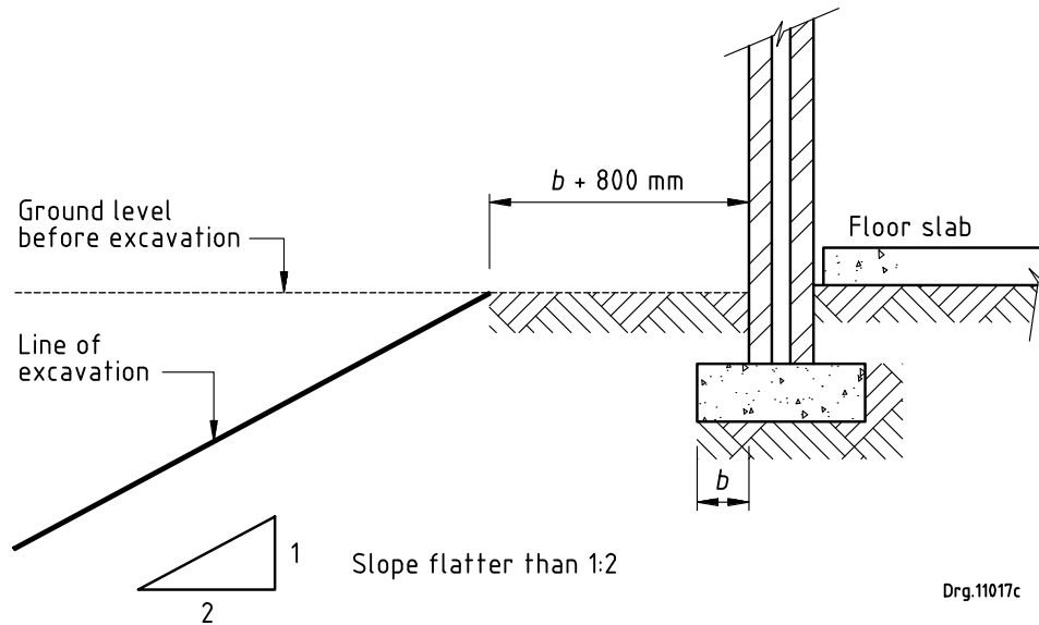
Figure 2 — Permanent excavations
