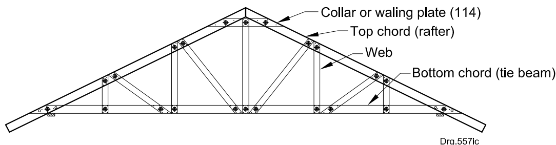
9(c) 6 Bay Howe Truss with 114 members
