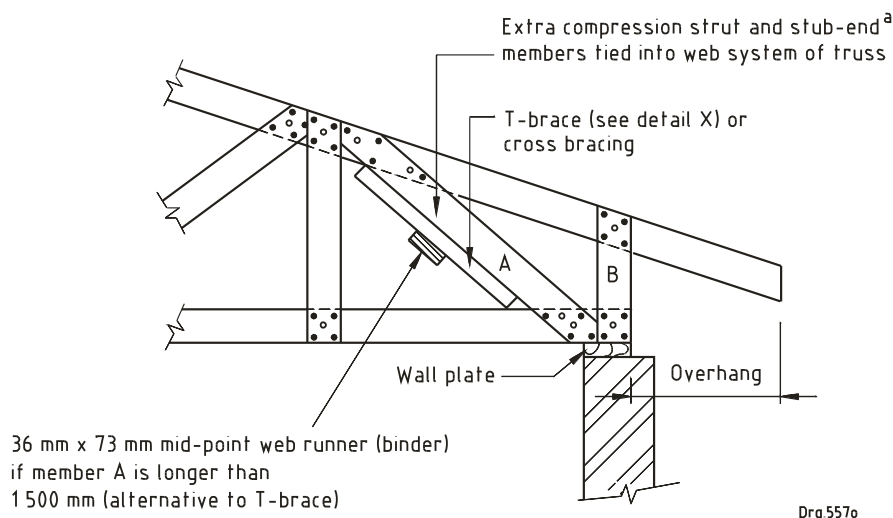
a) Stub-end trusses
