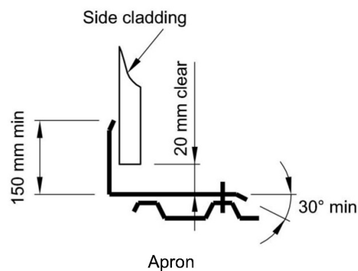
Figure B.2 — Transverse flashings
