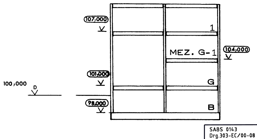
Fig. 15 – Method of Numbering Floors
