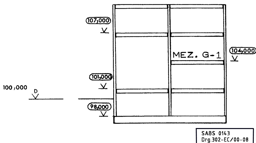
Fig. 14 — Levels on Section and Elevation
