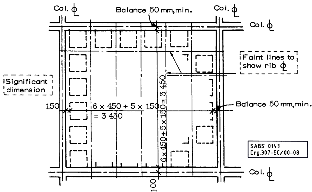
Fig. 20 ) Two-Way Rib Coffers or Filler Blocks
