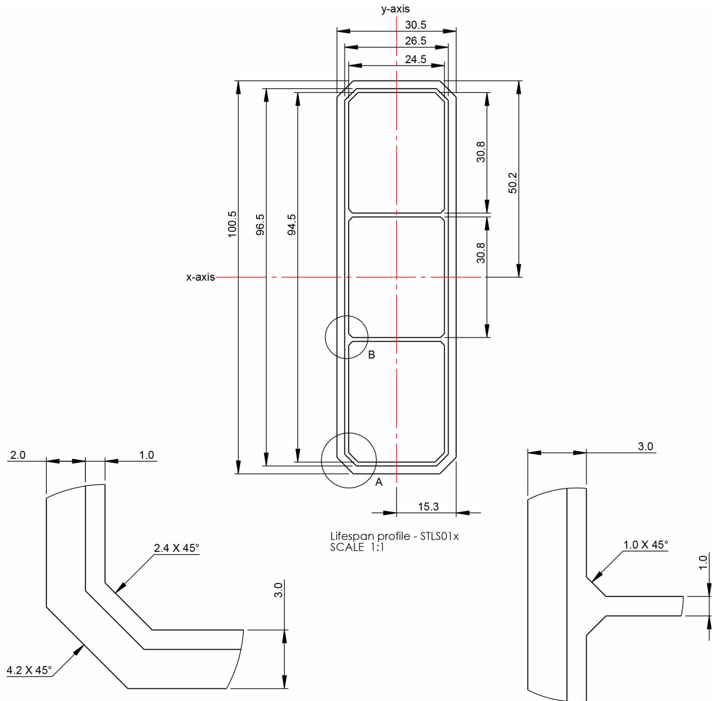
DETAIL A SCALE 5 : 1
