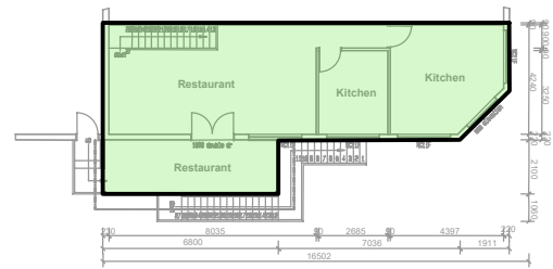
Main Building: Second Floor = 84m 2
