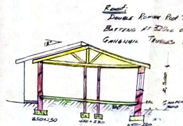
SECTION-B-B 1:100
