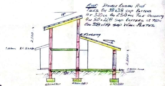
SECTION-C-C 1:100
