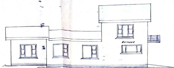
WEST ELEVATION 1:100
