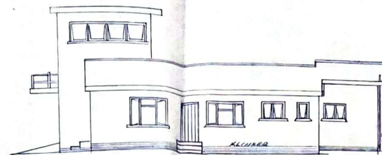
EAST ELEVATION 1:100
