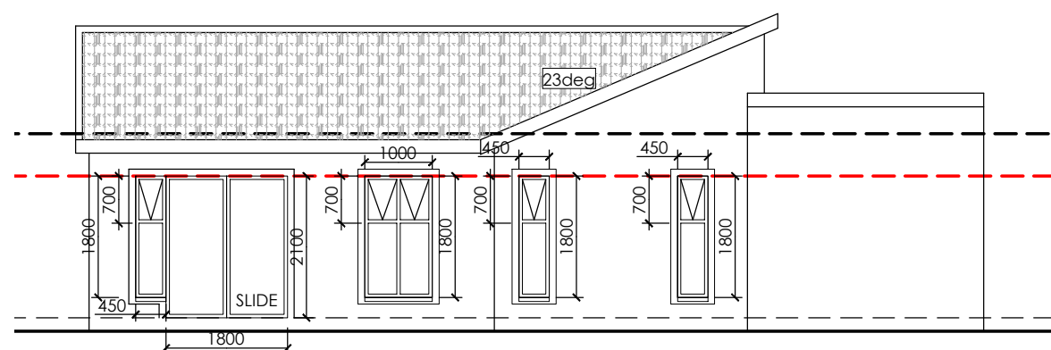
NORTH ELEVATION
