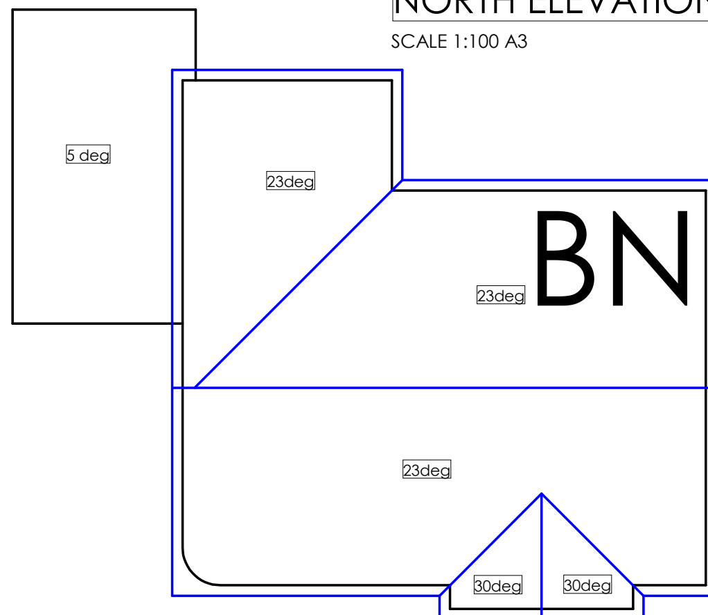
NORTH ELEVATION
