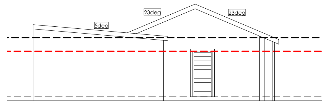
WEST ELEVATION
