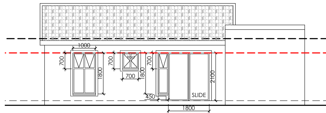
NORTH ELEVATION
