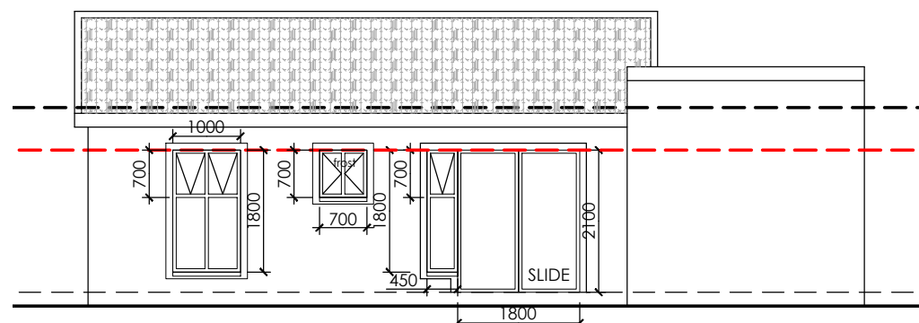
NORTH ELEVATION
