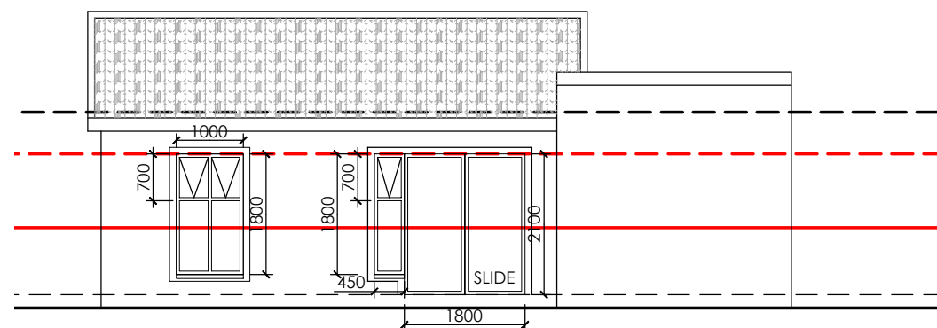
NORTH ELEVATION
