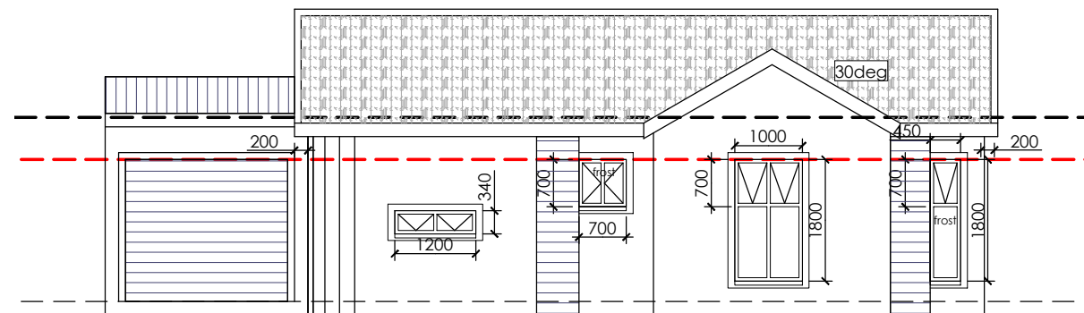
SOUTH ELEVATION
