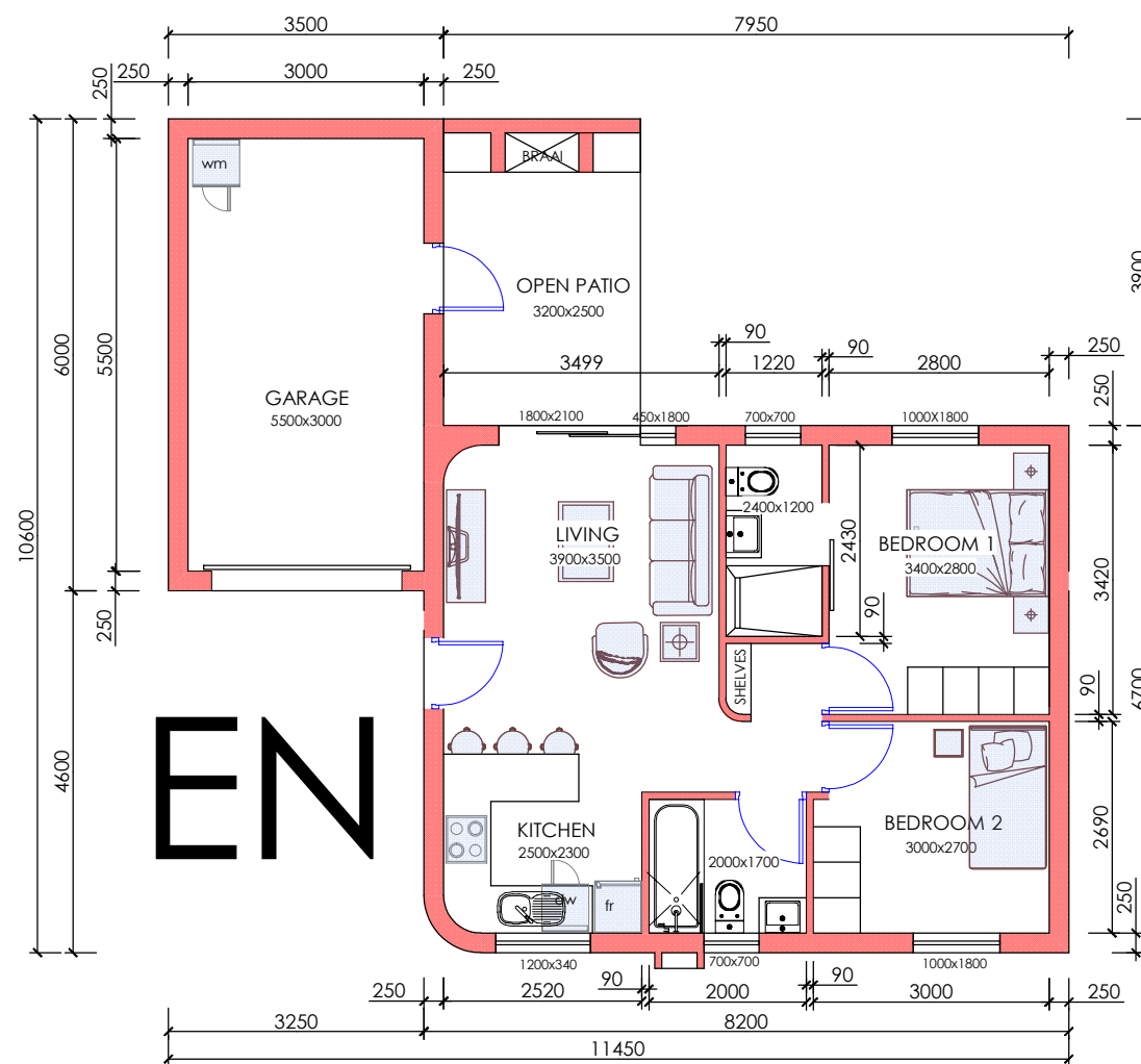
FLOOR PLAN SCALE 1:100 A3
