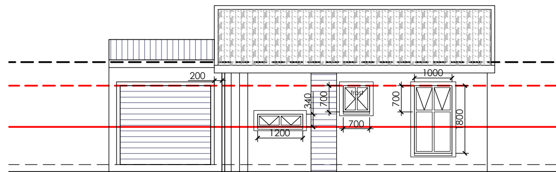
SOUTH ELEVATION
