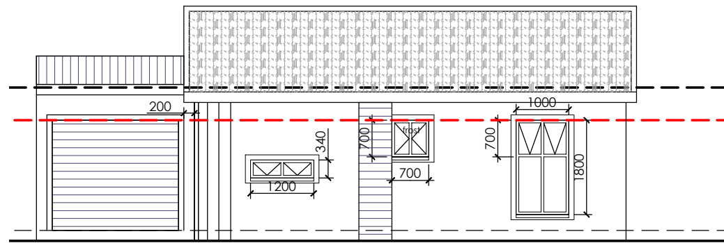
SOUTH ELEVATION
