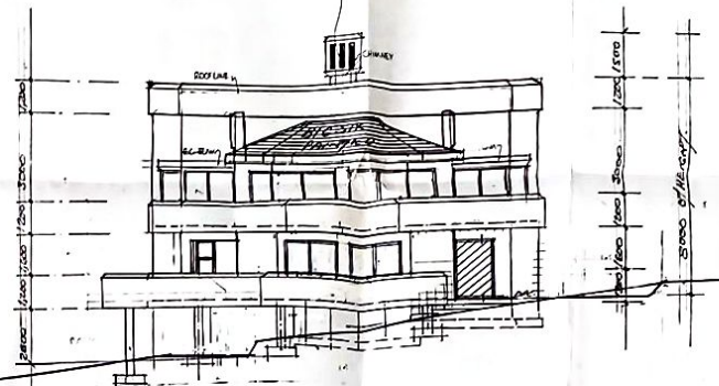
NORTH-EAST ELEVATION SCALE 1:100
